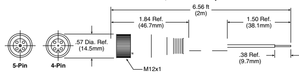
CB-M12-4P-2M, Female to Open Lead CB-M12-5P-2M, Female to Open Lead
